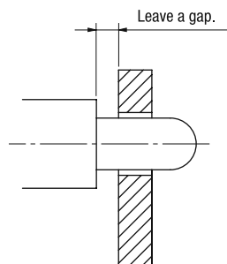
Figure 7: Example of Stepped Pin Usage
