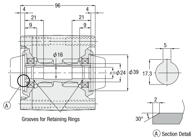
Detailed Dimension Chart for Hollow Shaft (mm)
