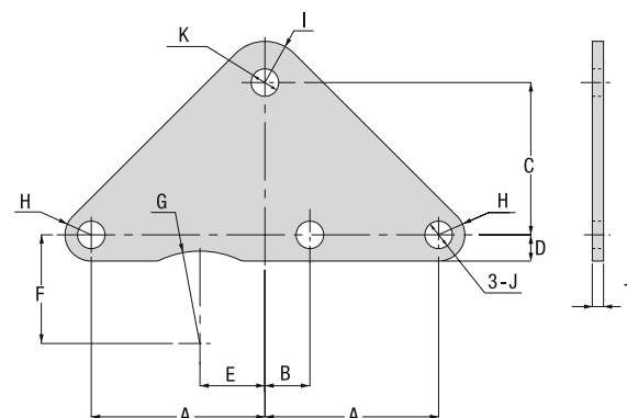
Frames 25–35
